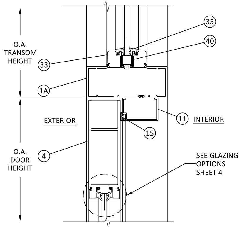
G 6 VERTICAL SECTION TRANSOM BAR AT DOOR HEAD OHCC
