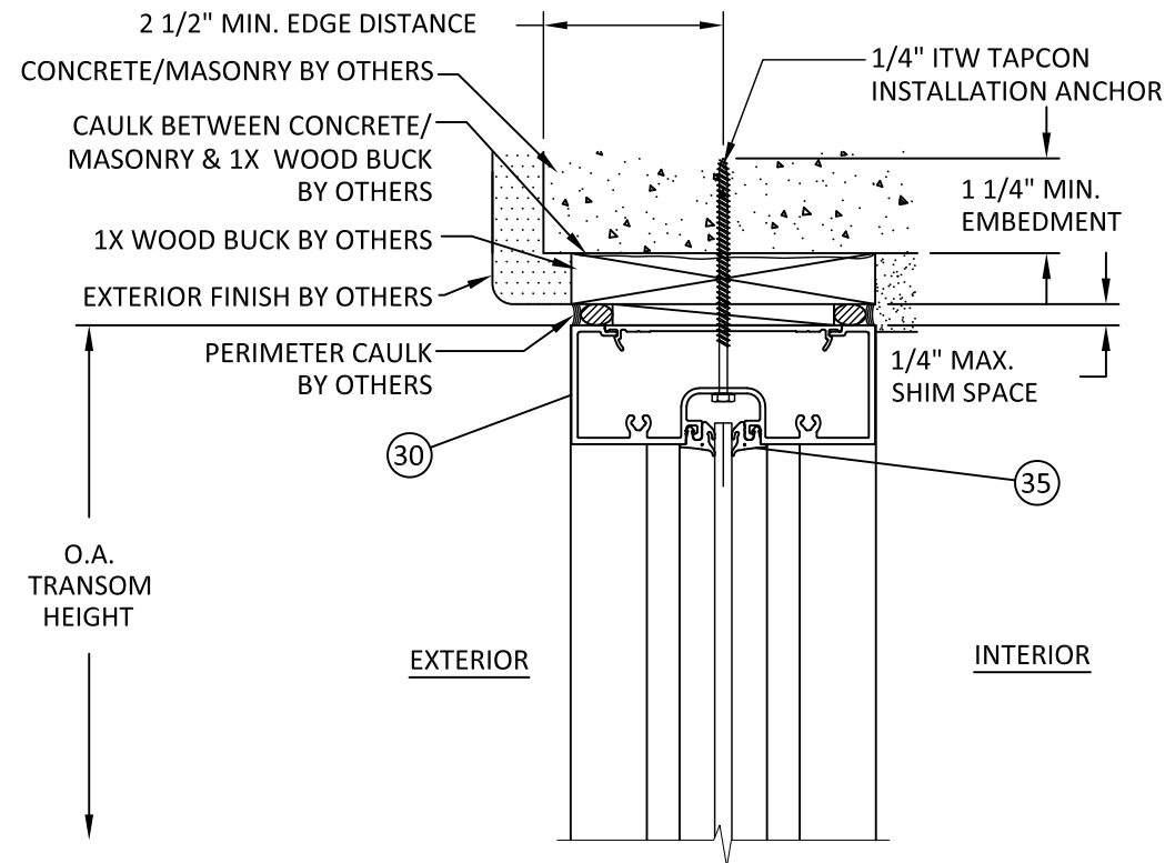
H 6 VERTICAL SECTION TRANSOM HEAD - CONCRETE/MASONRY
