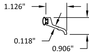
28 THRESHOLD STOP
