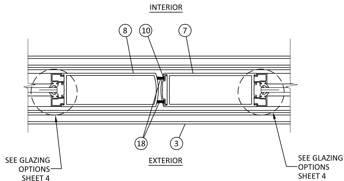
F 5 HORIZONTAL SECTION MEETING STILE
