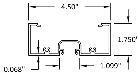
30 HEAD (MONO)
