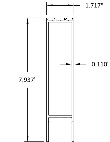
5A 8" BOTTOM RAIL
