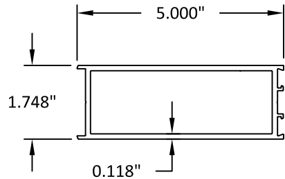
7 MEETING STILE (ACTIVE)
