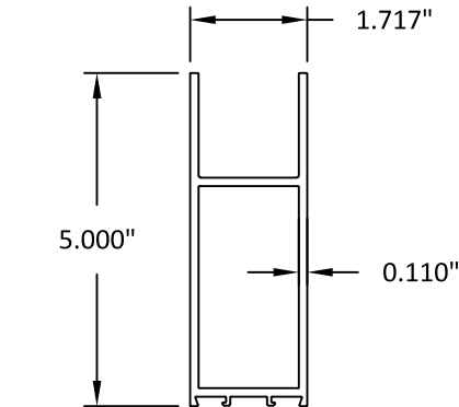
4 TOP RAIL
