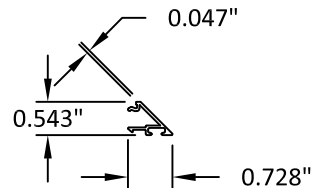
13 1/4" BEVELED GLASS STOP
