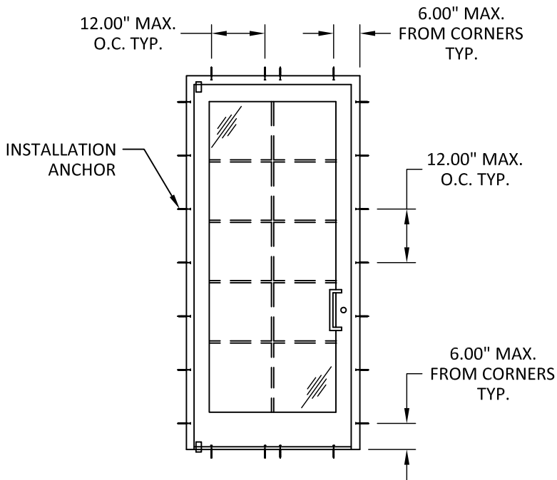
ANCHOR LAYOUT
