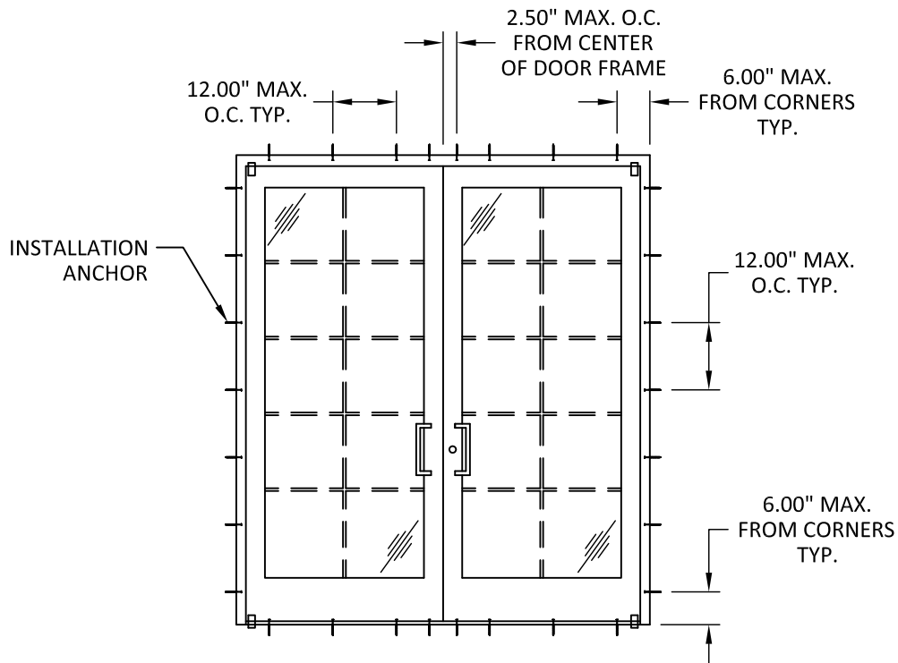
ANCHOR LAYOUT
