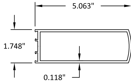
8 MEETING STILE (INACTIVE)
