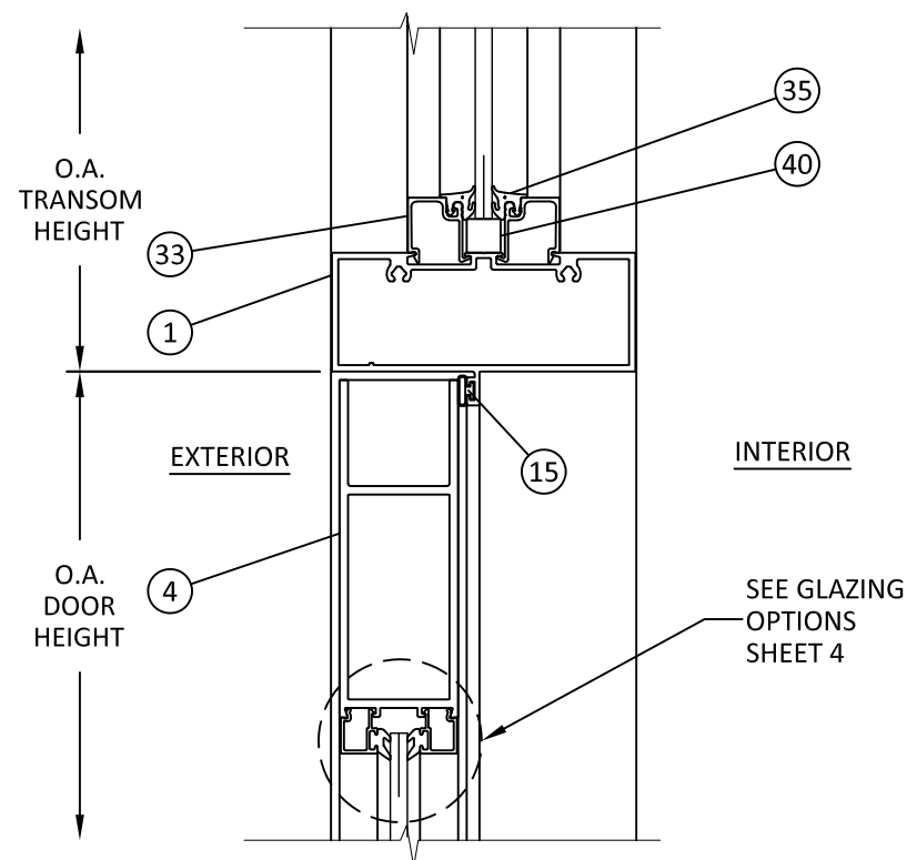
G 6 VERTICAL SECTION TRANSOM BAR AT DOOR HEAD
