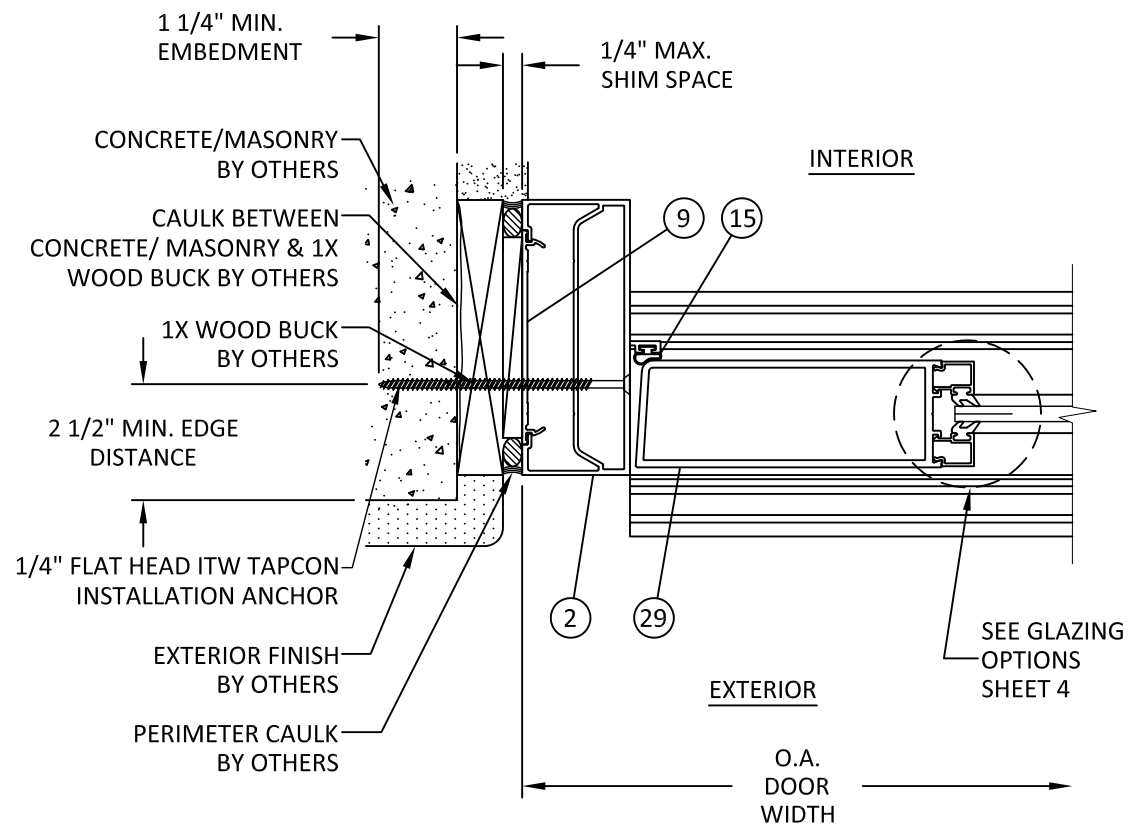
D 5 HORIZONTAL SECTION JAMB - CONCRETE/MASONRY
