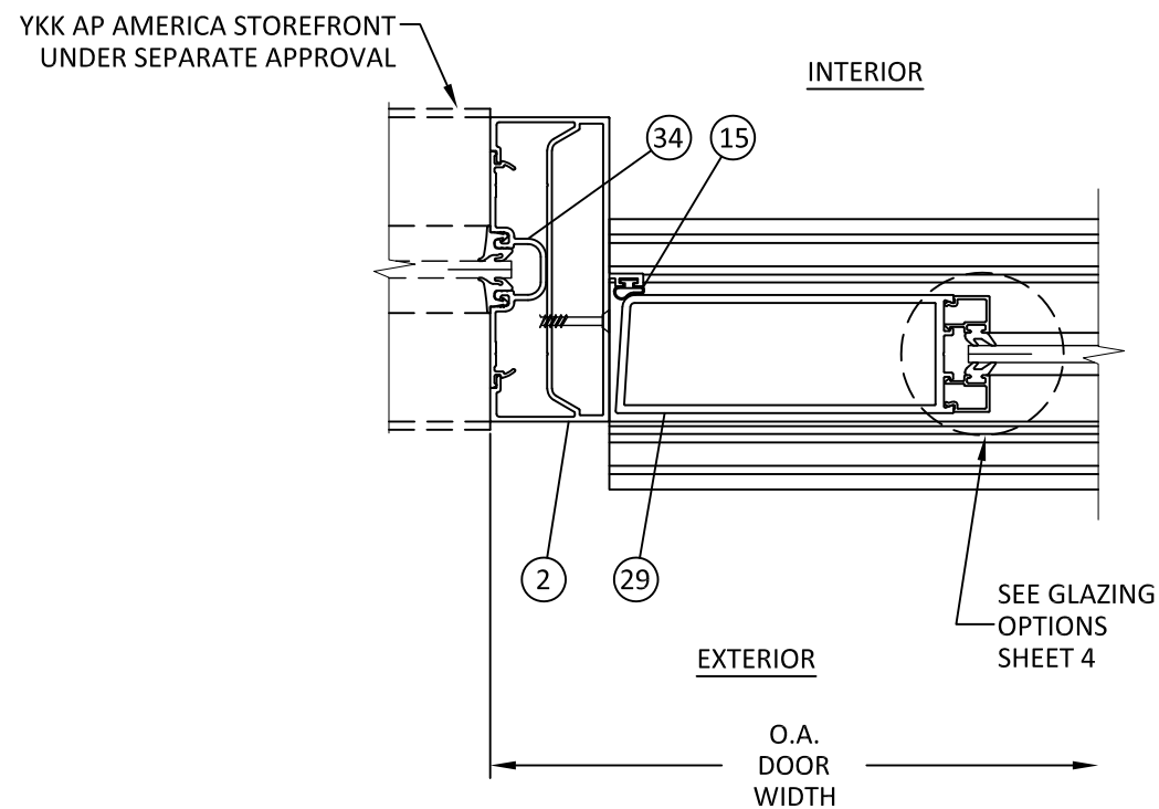
L 5 HORIZONTAL SECTION JAMB - STOREFRONT INSTALLATION
