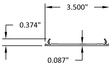
9 FLAT FILLER
